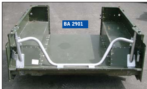
BA 2005 – Standard Roll Cage
